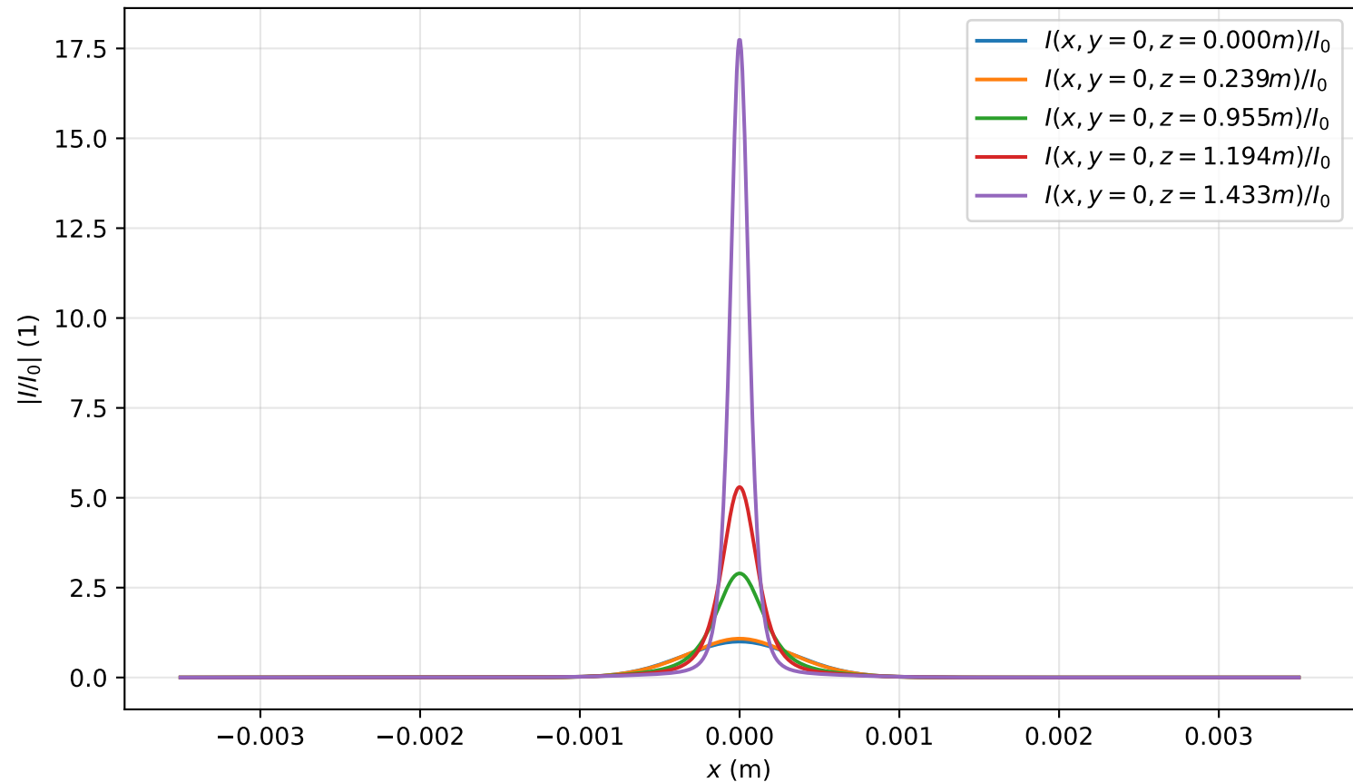
Intensity profile I(x, y = 0, z)/I_0 , P_{in}=1.6P_{cr} , artificial time
